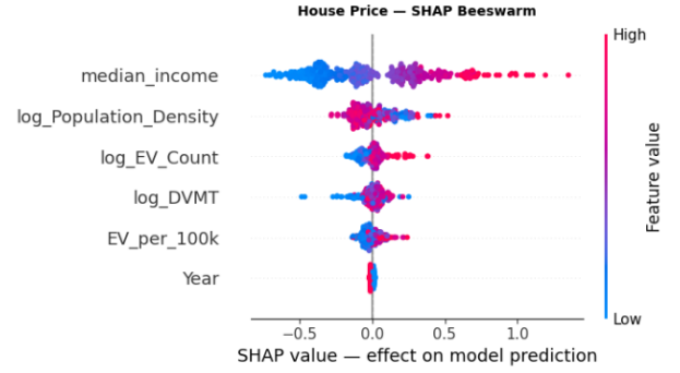
Figure 10. SHAP summary (beeswarm) plot for the XGBoost house price prediction model. The distribution of SHAP values illustrates the contribution of each feature across all observations, while the color indicates the corresponding feature value.
