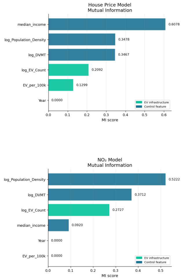
Figure 3. Mutual Information scores for the candidate predictors with respect to the target variable. Higher scores indicate greater relevance for predicting the response.
