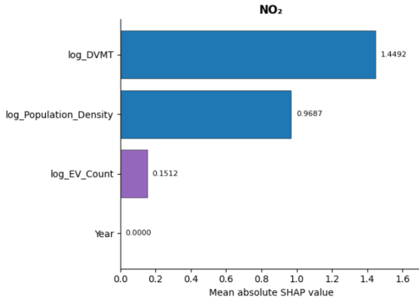
Figure 7. Global SHAP feature importance for the XGBoost NO 2 prediction model. Feature importance is measured as the mean absolute SHAP value.
